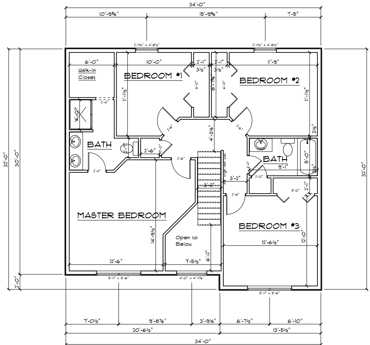
Two Story 2nd Floor Plan
